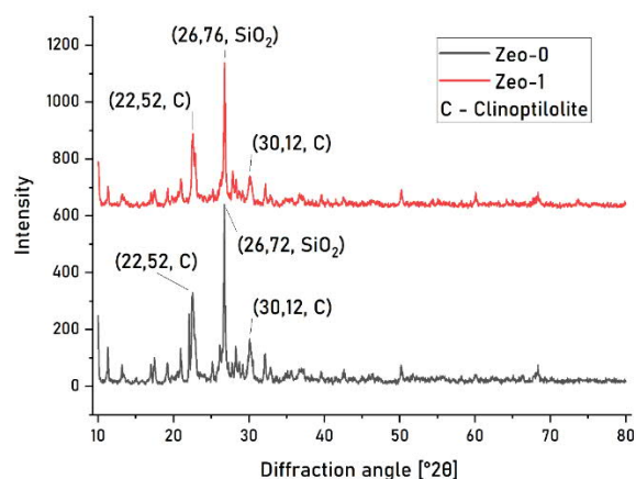
Fig. 1. X-ray phase analysis of natural and acid-activated zeolite
